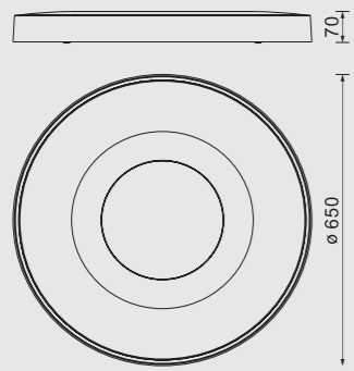
7691 Arena-Sabbia LED 80W 2700K-5000K 3900lm
