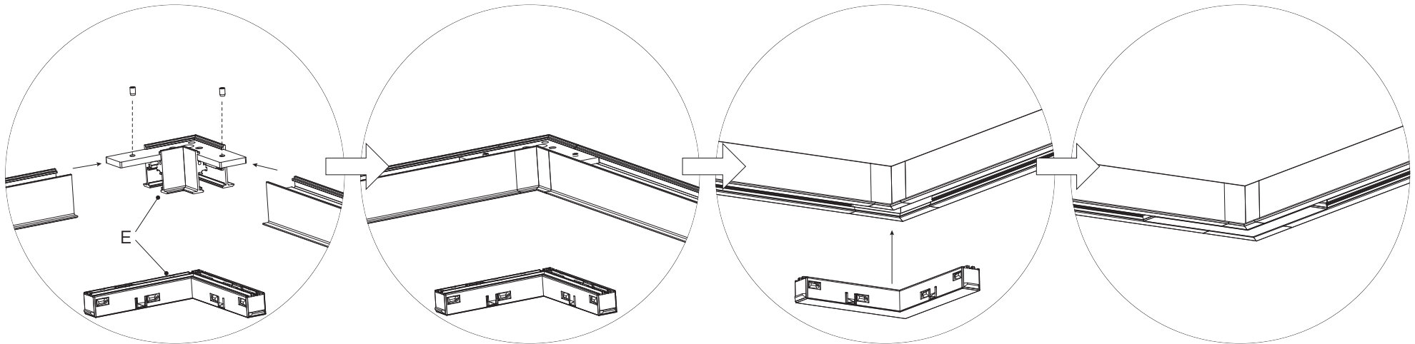
L-connector
