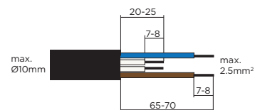
cable specification
